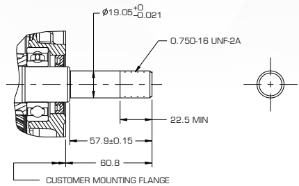
3/4" 螺纹轴
