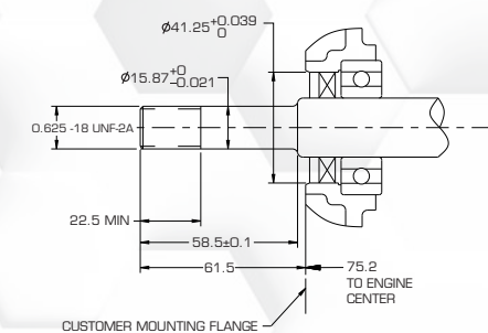
5/8" 螺纹轴
