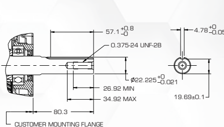
7/8" 键槽轴
