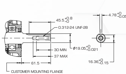
3/4" 键槽轴
