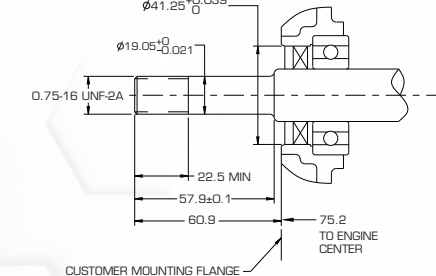
3/4" 螺纹轴
