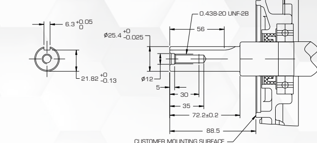
1" 键槽轴
