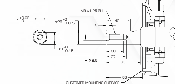
25mm 键槽轴
