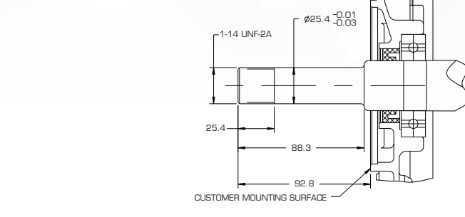
1" 螺纹轴
